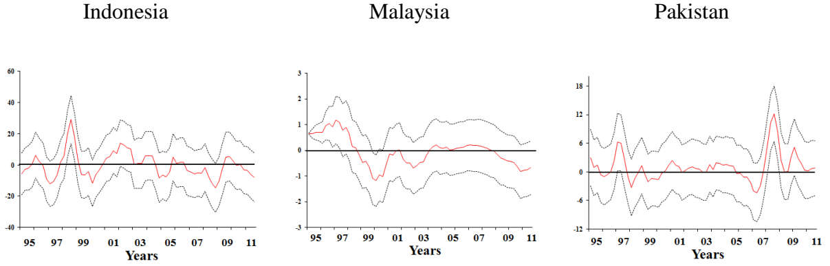
Figure 1: IREG and 2× st.dev. bootstrapped confidence intervals
